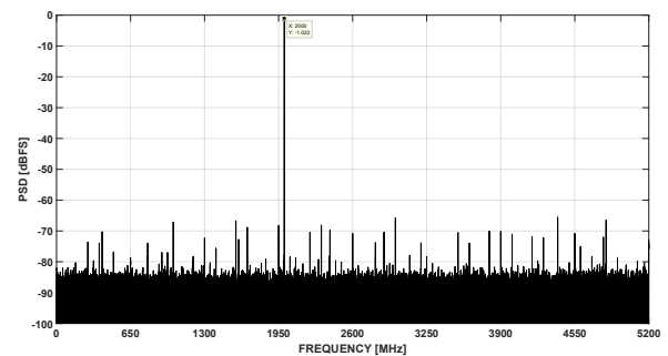
图 7-4. FFT at F_{in} = 2\text{GHz} , 10.4GSPS (0.5Vpp FS, -1 dBFS)
